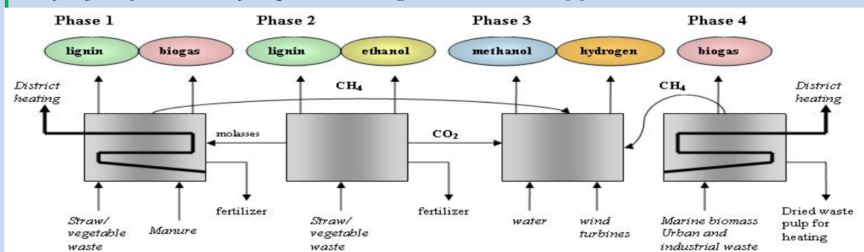
Biorefinery Platform: Phases of the process. The diagram created based on [9]
